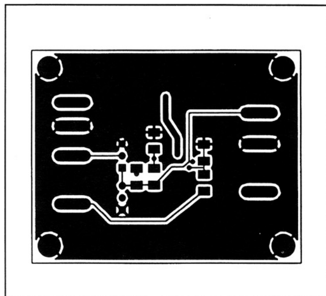
Figure 5. MAX866 EV Kit PC Board Layout—Solder Side
