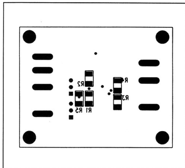
Figure 3. MAX866 EV Kit Component Placement Guide—Solder Side
