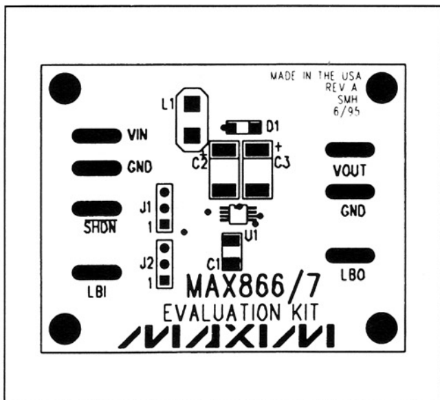
Figure 2. MAX866 EV Kit Component Placement Guide—Component Side
